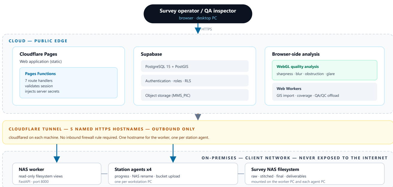
Figure 2. System architecture. The browser never receives an on-premises credential — Pages Functions validate the session and inject server-side secrets before proxying. The NAS is reachable only by the worker and the agents.
